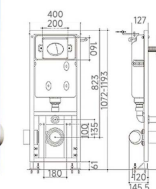
OY-100 Concealed Water Tank
